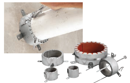
3M ™ Fire Barrier Ultra Plastic Pipe Device: Can be used to firestop a variety of plastic pipes which include ccPVC, PVC, CPVC, ccABS, ABS, FRPP and PVDF.
